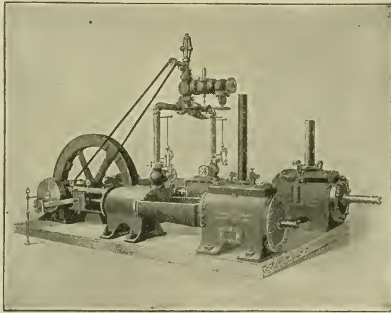
INGERSOLL-SERGEANT DUPLEX STEAM-ACTUATED AIR COMPRESSOR.
